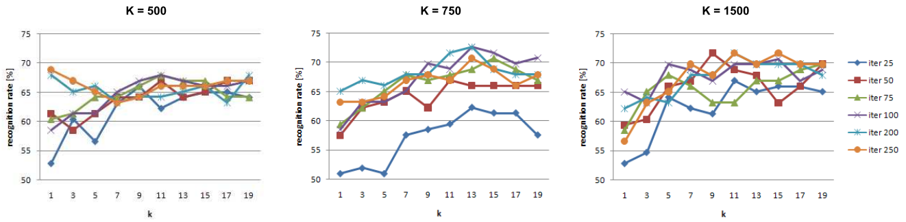
Figure 7: Recognition rates of the FSGW-pLSA on the validation set for various k 's of the kNN algorithm, different numbers of iterations of the EM algorithm, and different numbers of Gaussians K in the model.
