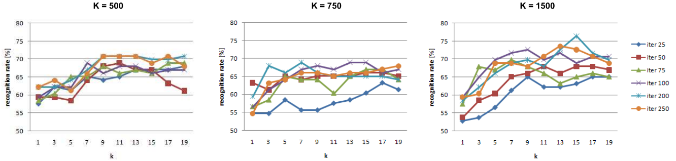
Figure 5: Recognition rates of the original pLSA model on the validation set for various k 's of the kNN algorithm, different numbers of iterations of the EM algorithm, and different numbers of visual words K in the model.
